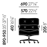
Lobby Chair ES 104
